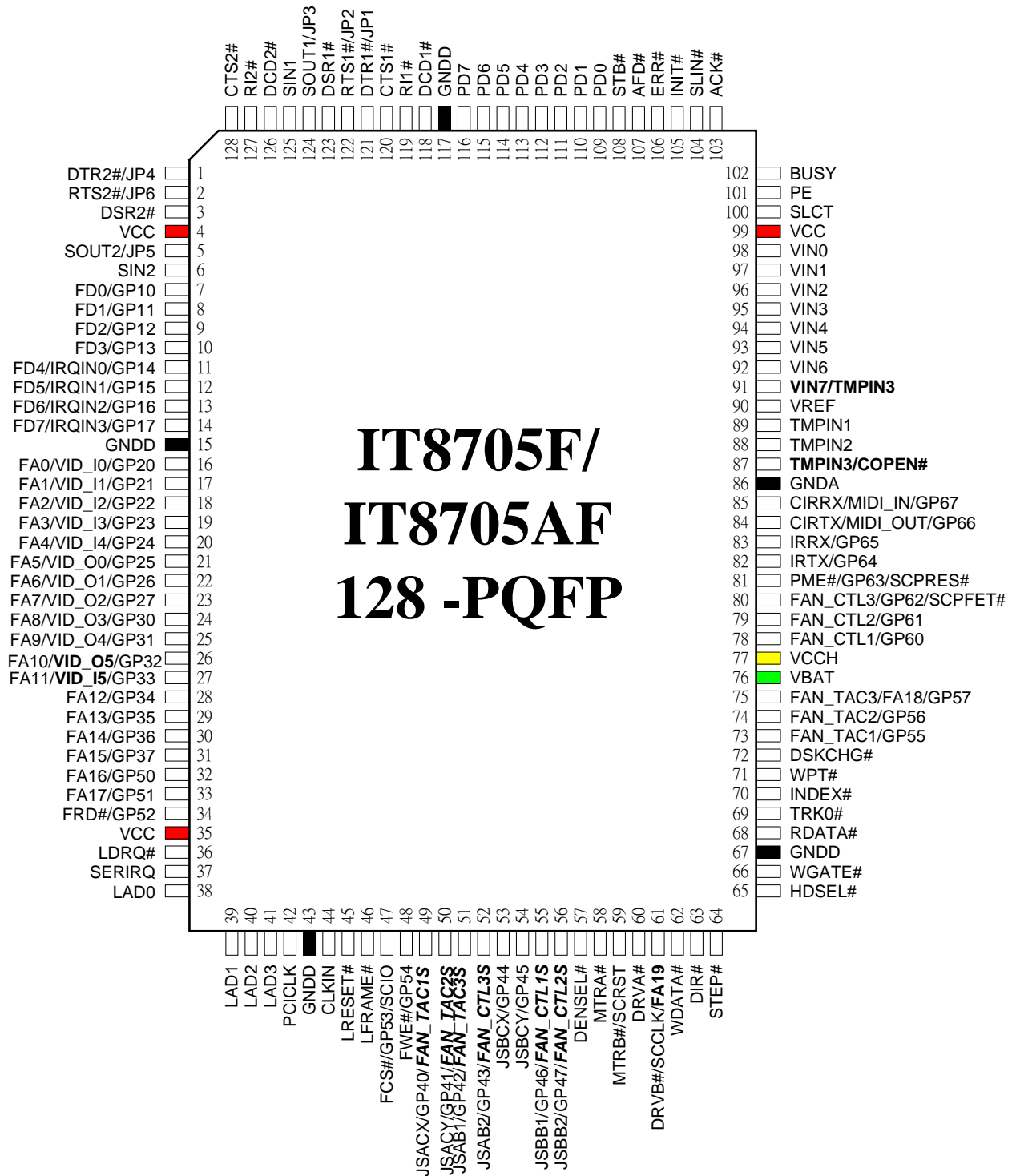
Top View
