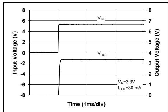
FIGURE 2-35: Startup Response.
