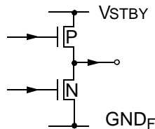
Fig. 4-10: Output pin CLK5
