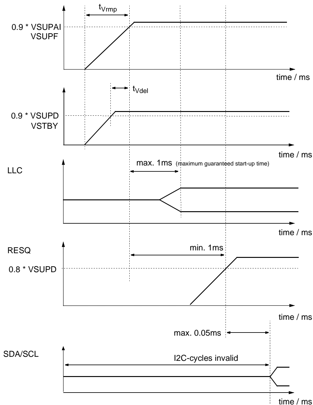
Fig. 4-13: Power-Up sequence
