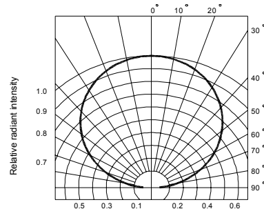
Fig.6 Radiation diagram
