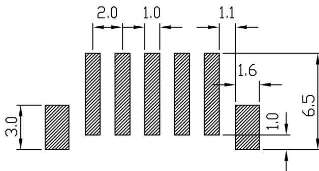
RECOMMENDED P.C.BOARD PATTERN DIM.
