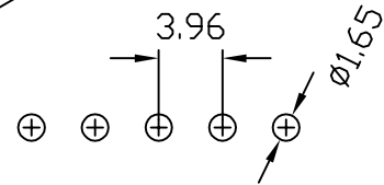
RECOMMENDED P.C.BOARD HOLE DIMM.
