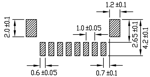
RECOMMENDED P.C.BOARD PATTERN DIM.
